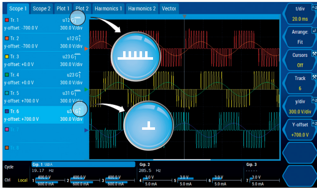
Scope display of the voltages at the converter output. The wideband values (jagged waveform) show the PWM signal, the narrowband values (smooth waveform) are sinusoidal.
